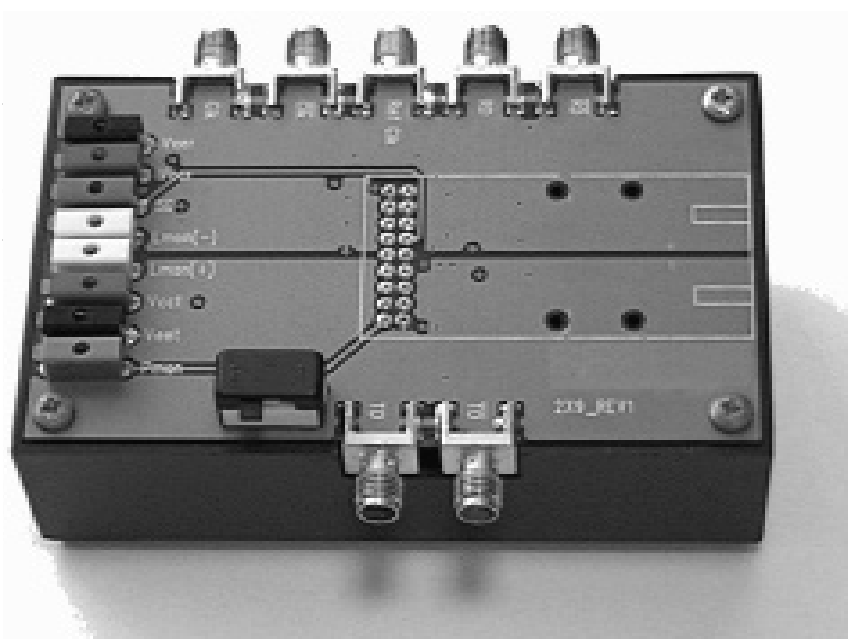
Figure 10. HFCT-5000 Evaluation Board
